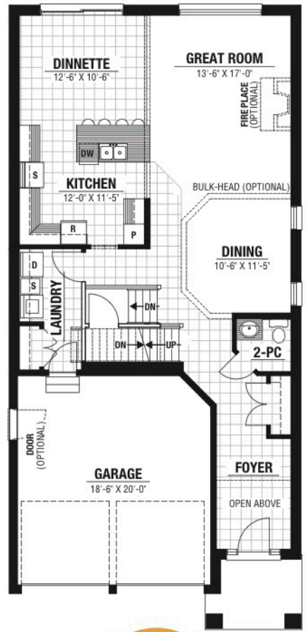
MAIN 1142 sq. ft.
