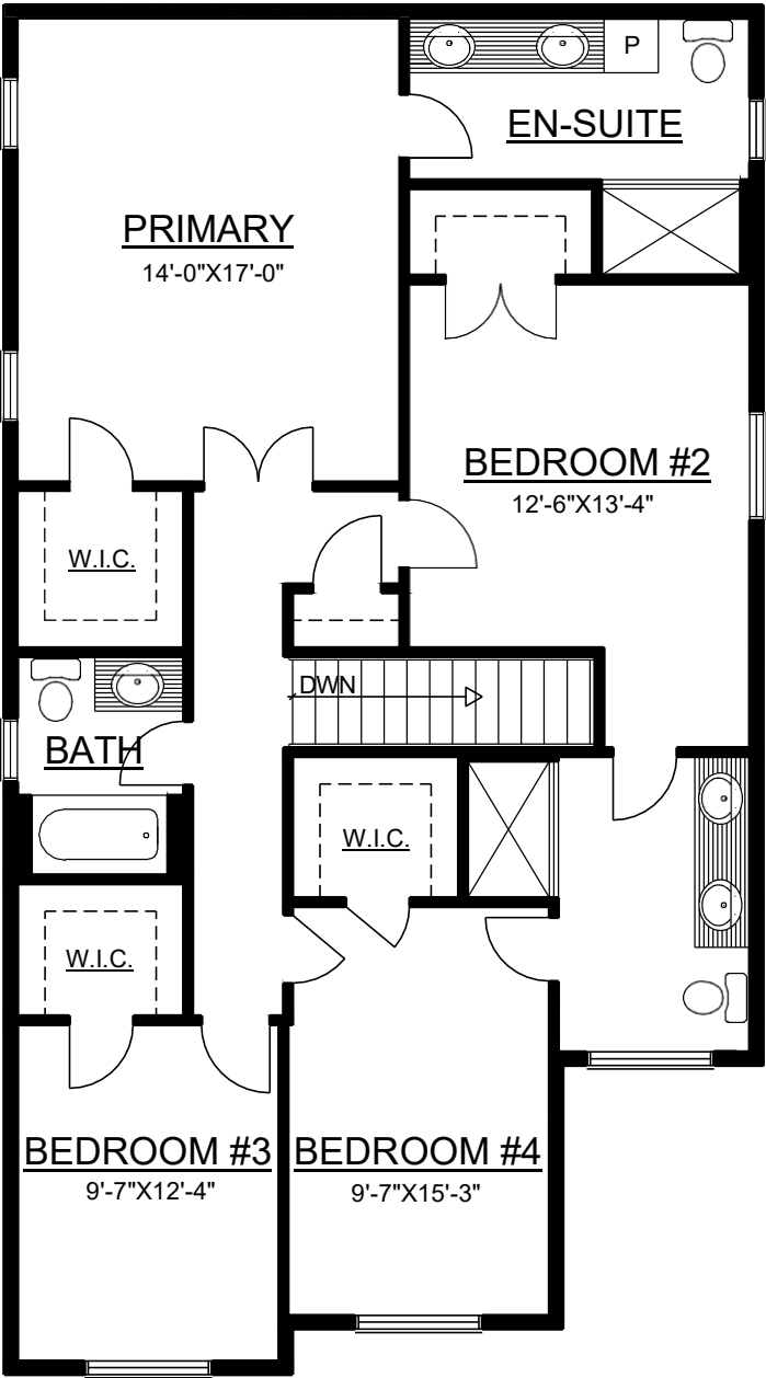
BAYFIELD PLUS SECOND FLOOR PLAN OPT 1 APPROX 1299 SQ. FT.
