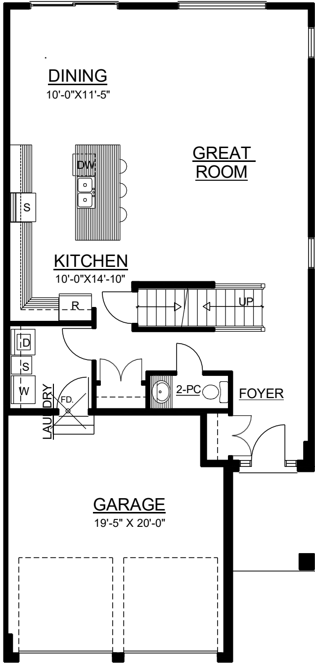
BAYFIELD PLUS FIRST FLOOR PLAN APPROX 1017 SQ. FT.
