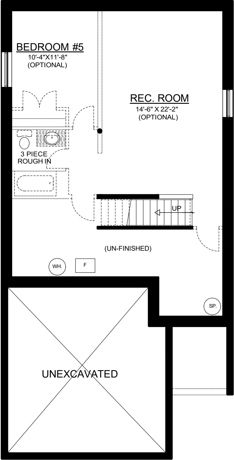
"BAYFIELD PLUS" FOUNDATION PLAN APPROX. 667 SQ. FT. OF OPTIONAL FINISHED BASEMENT APPROX. -2316 TOTAL SQ. FT.
